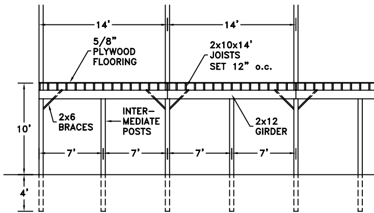
LOFT FRAMING DETAIL
