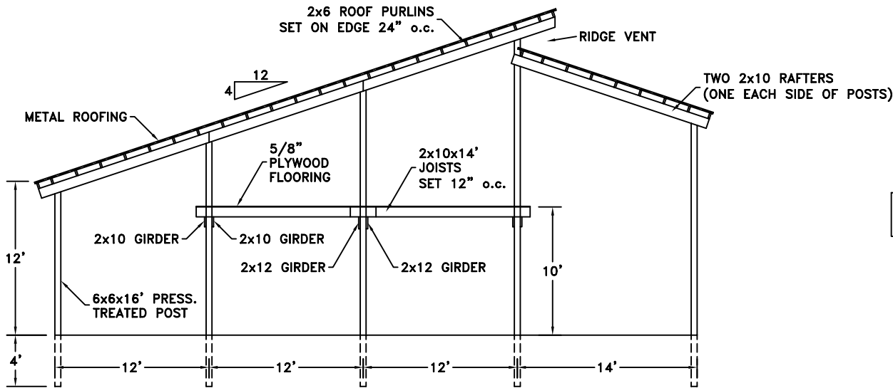
CROSS SECTION
