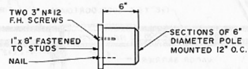
BRIDLE RACK
