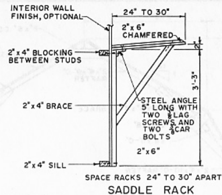
SADDLE RACK
