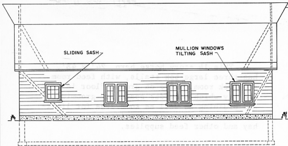
SIDE ELEVATION
