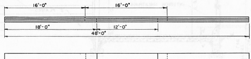
GIRDER LAMINATION DETAIL
